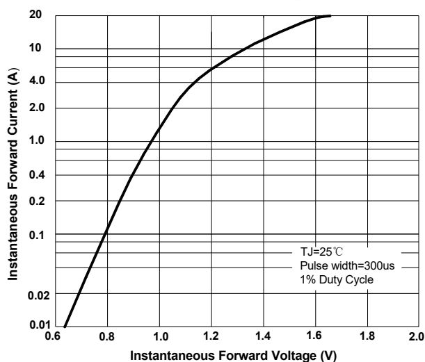
FIG.3: Forward Voltage
